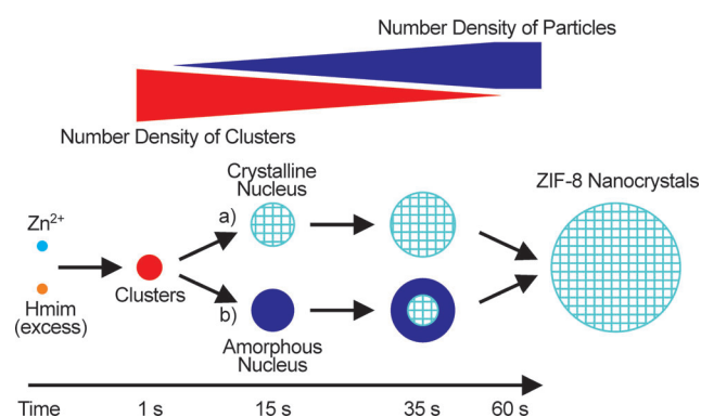
Scheme 1. Species occurring during nucleation and growth of ZIF-8 nanocrystals under conditions of high supersaturation. Two possible alternative crystallization pathways (a) and (b) are considered.
